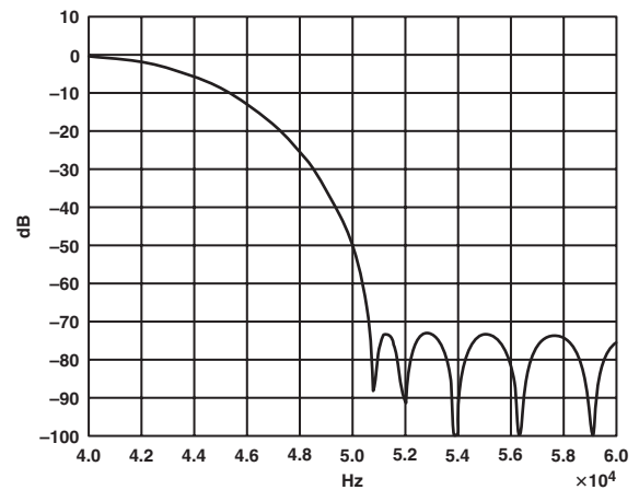
TPC 6. Transition Band Response, 4 \times Mode
