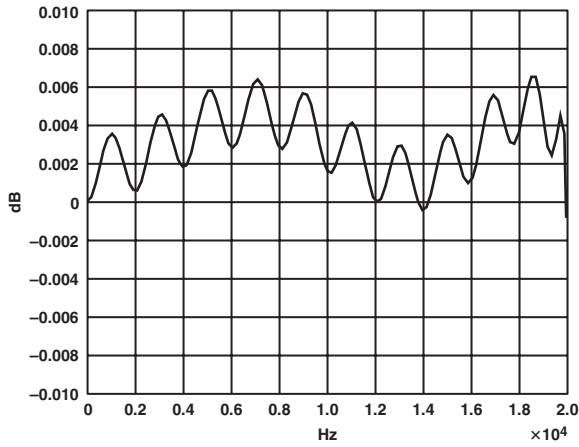
TPC 1. Pass-Band Response, 8 \times Mode
